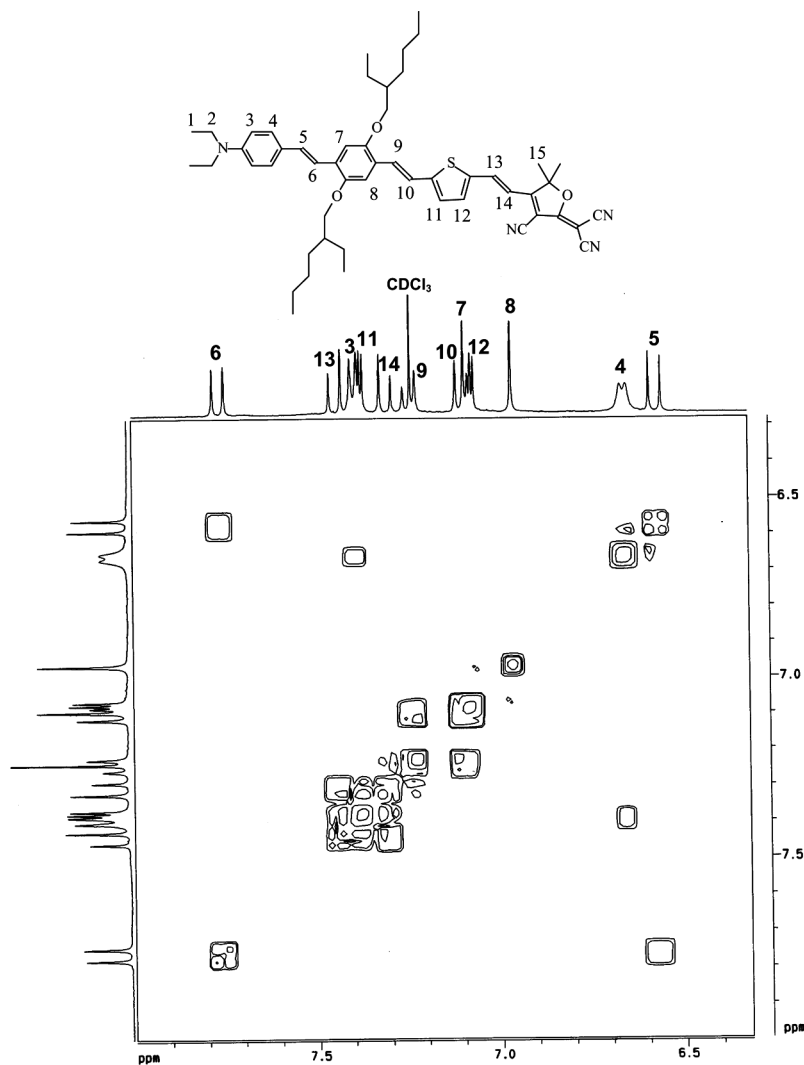
FIGURE 2 ^1\text{H} - ^1\text{H} COSY NMR spectrum of PT-TCF at 500 MHz.
