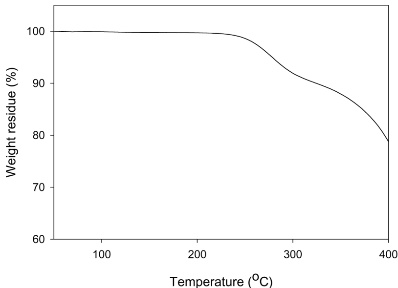
FIGURE 3 TGA thermogram of PT-TCF.
