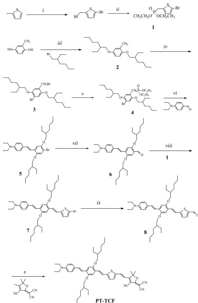
SCHEME 1 Synthesis of the NLO chromophore PT-TCF. Reaction conditions: (i) NBS, BPO, \text{CCl}_4 , 20 h, reflux; (ii) triethyl phosphite, 16 h, 160^\circ\text{C} ; (iii) acetonitrile, \text{K}_2\text{CO}_3 , reflux, 3 days; (iv) (a) NBS, AIBN, \text{CCl}_4 , 2 h, reflux and (b) NBS, THF, 1 h, reflux; (v) triethyl phosphite, 2 h, 160^\circ\text{C} ; (vi) NaH, THF, 0^\circ\text{C} for 15 min and reflux for 11 h; (vii) butyl lithium, DMF, THF, 3 h, rt.; (viii) LDA, THF, 5 h, rt.; (ix) butyl lithium, DMF, THF, 16 h, rt.; (x) piperidine, THF, overnight, rt.
