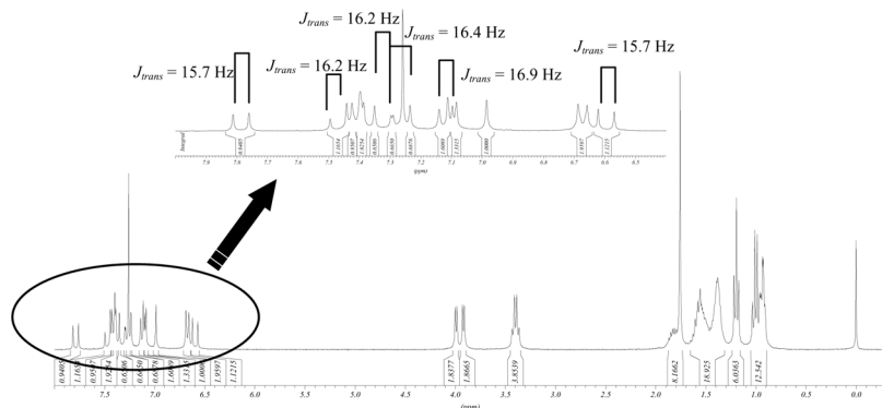
FIGURE 1 ^1\text{H} NMR spectrum of PT-TCF.
